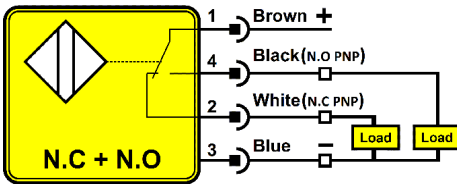
4 Pins Male Connector
